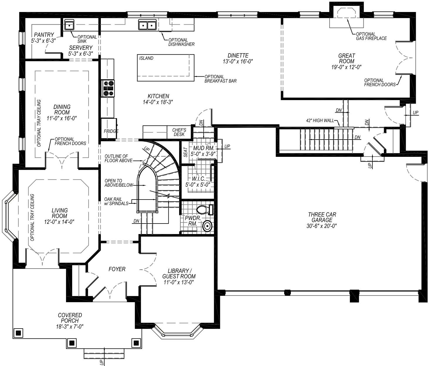
Main Floor Plan Approximately 4,000 sq.ft. Approximately 62'-0" x 50'-6" Optional 9'-0" ceiling
